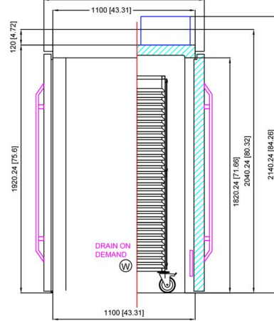
SIDE VIEW SECTION WITH BOTTOM
