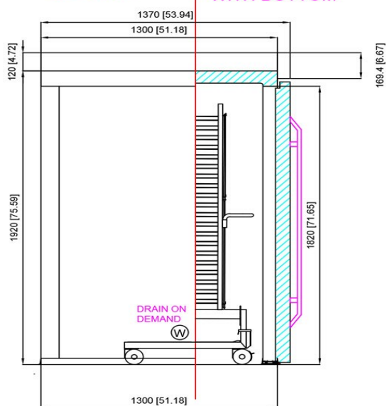
SECTION B-B WITH BOTTOM
