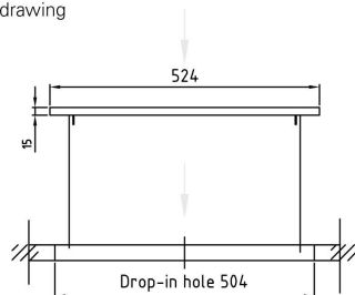
Mounting drawing
